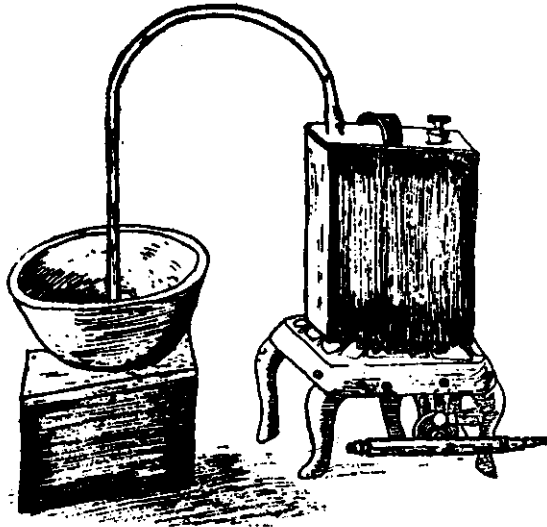
FIG. 57. APPARATUS FOR CLEANING SKELETONS. THE BOWL CONTAINS SODIUM SULPHIDE SOLUTION WITH STEAM PLAYING INTO IT THROUGH THE PIPE.
