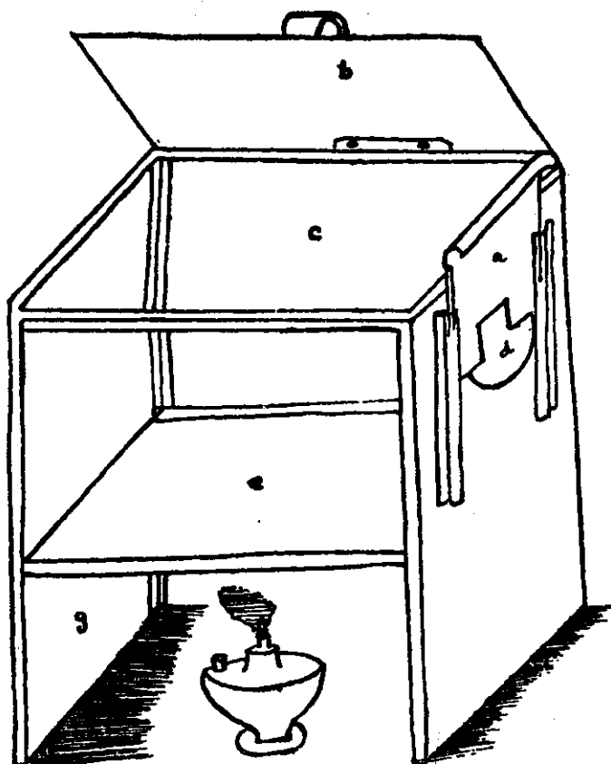
FIG. 17. APPARATUS FOR BLOWING INSECT LARVAE. a. SIDE SHUTTER; b. LID; c. BACK PANEL; d. OPENING FOR INTRODUCING THE LARVA; e. BOTTOM PANEL; f. SPIRIT LAMP; g. STAND.
